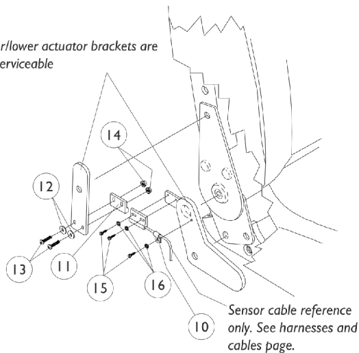
Actuator Attaching Hardware (High Back 18" Wide Models Only)
