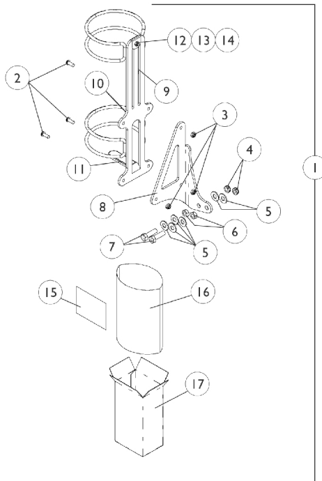
Installing on Seat with Internal Hinge
