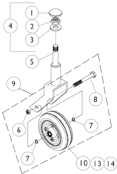
6" Caster Assembly
