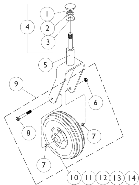
8" Caster Assembly
