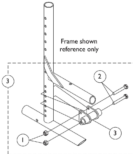
Chairs built Before 6/24/99
