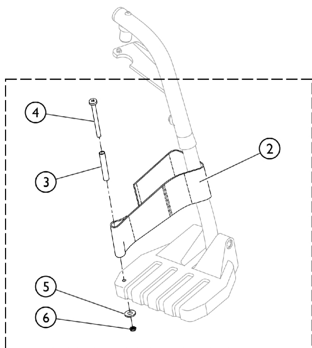
① Heel Loop and Hardware for All Footplate Options (Except Deluxe I450)
