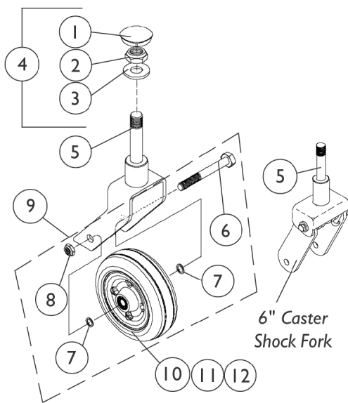
6" Caster Assembly
