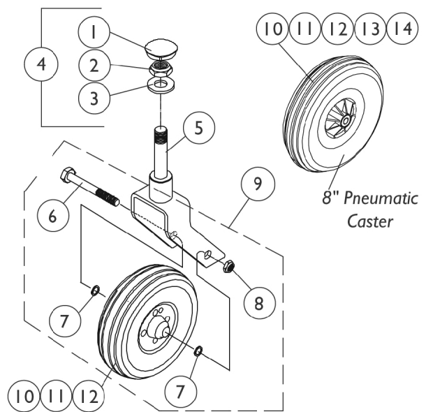
8" Caster Assembly
