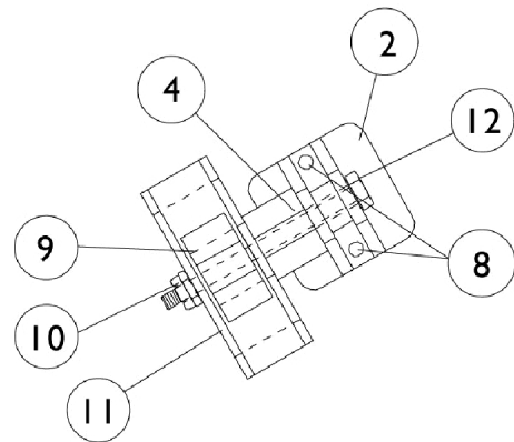
PAL4A/PAS4A Articulating Legrest
