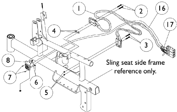
Battery Harness Layout (Sling Seat w/o Shrouds.)
