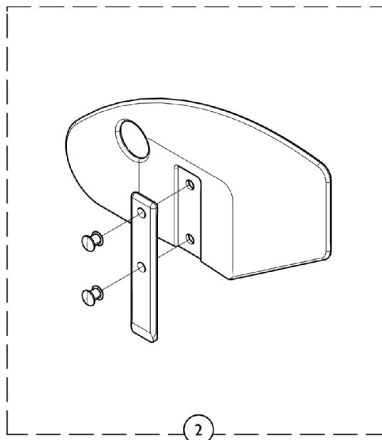
Small Rigid Guard (Shown w/ Quad Hole)
