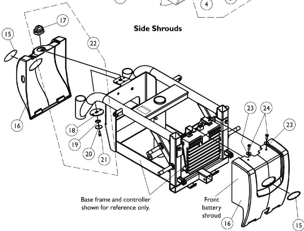
Front and Rear Battery Shrouds
