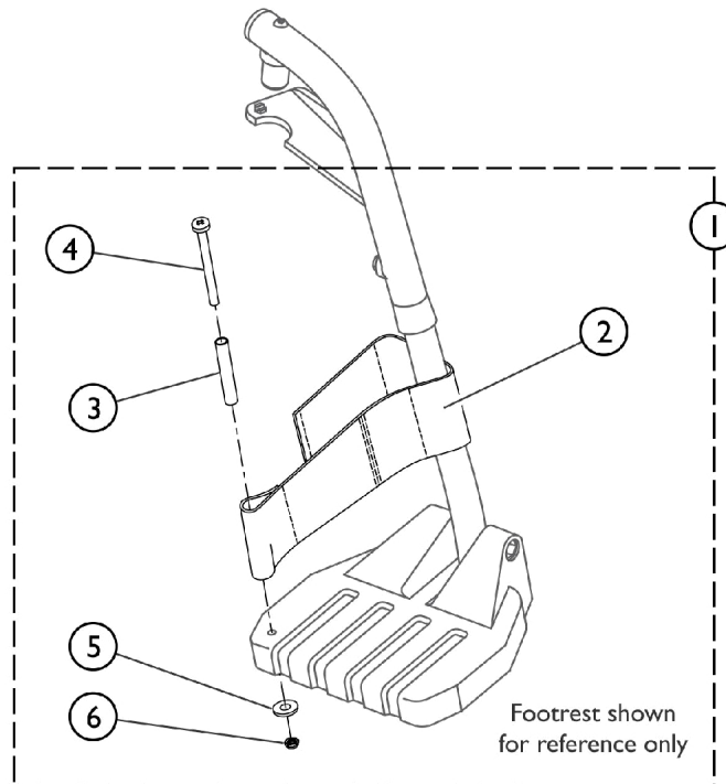
Heel Loop and Hardware for All Footplate Options with Toe Loops (1345) being used (not shown).
