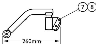
Anti-Tipper Configuration Chart
