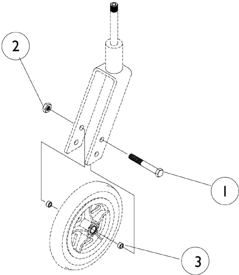
Caster Hardware
