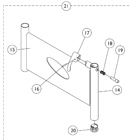
SARMHT - Standard (Low) Height Arm Base Assembly
