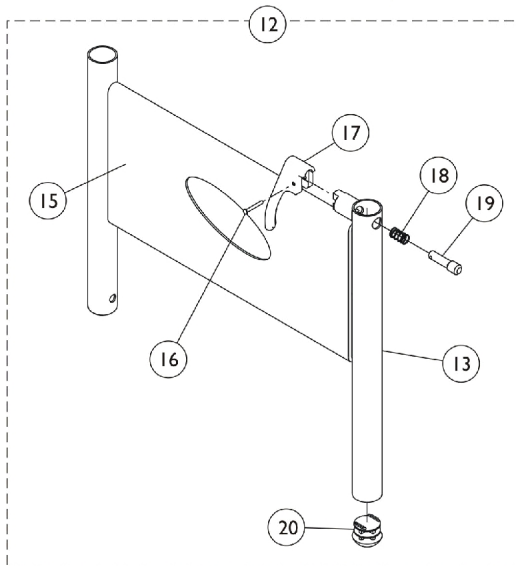
HARMHT - High Height Arm Base Assembly
