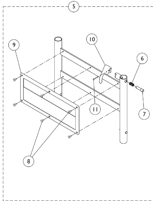
Adjustable Arm Base - Non-Flip Back
