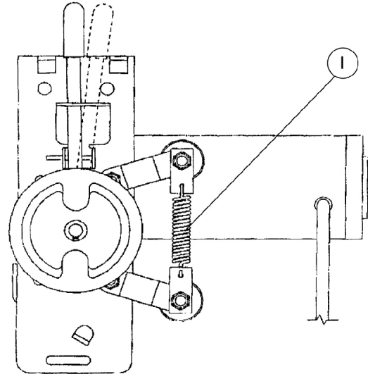
Auto Belt Tensioning System After 6/9/94
