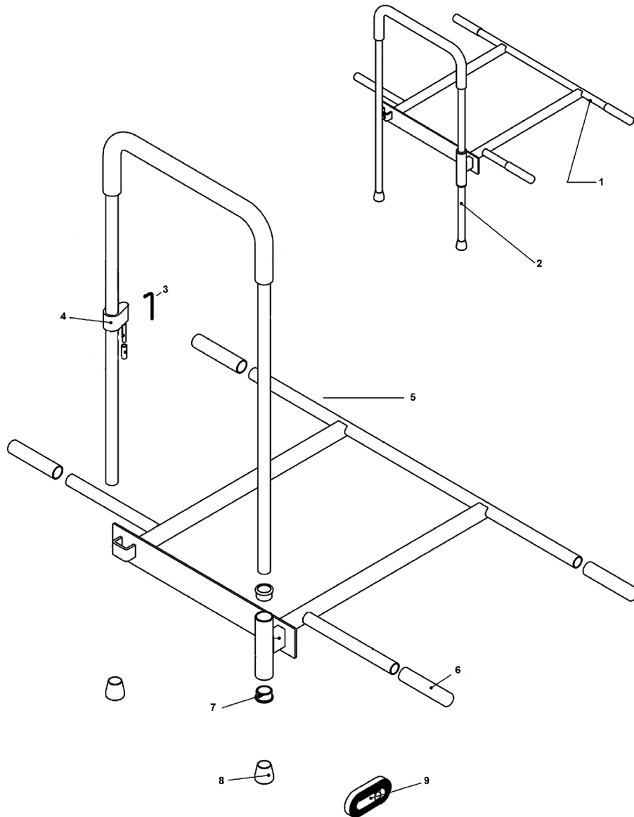
PARTS DIAGRAM: SMART-RAIL
