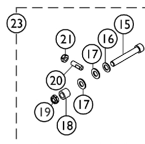
Detail "A" Footboard Mounting Hardware
