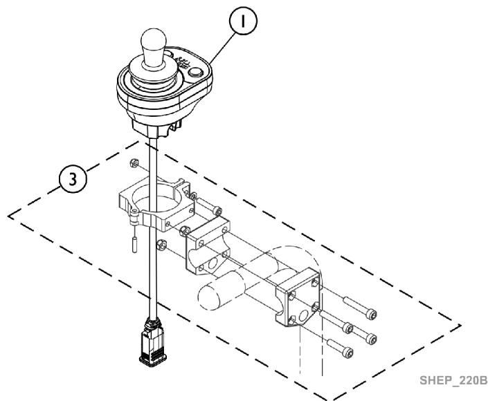
LiNX DLX-ACU200 ULMT/ASBA-2 Back Cane Mounting Hardware
