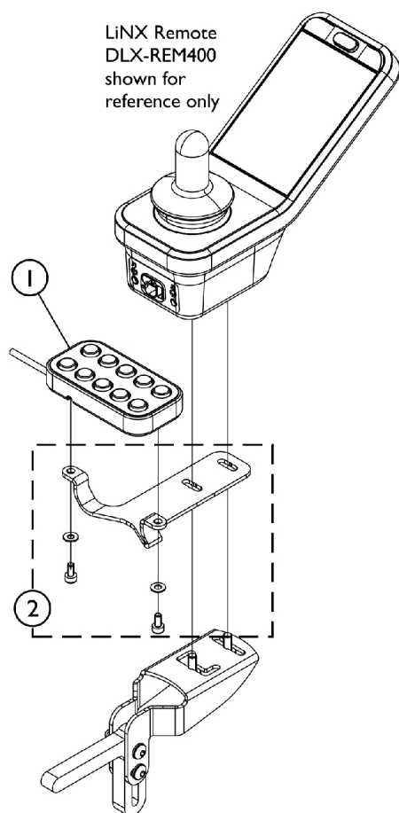
Remote Bracket Assembly shown for reference only
