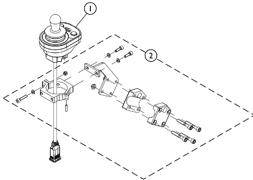
LiNX DLX-ACU200 ULMR/ULMTR Spreader Bar Mounting Hardware
