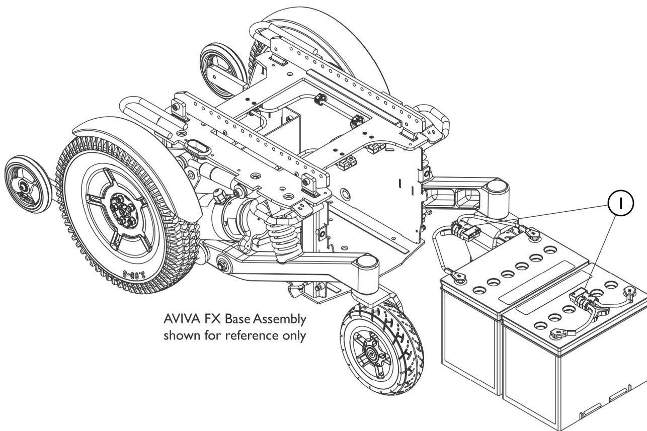
Batteries shown for reference only
