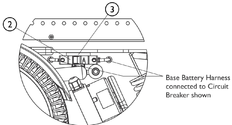
Assembled view of Circuit Breaker Assembly shown for reference
