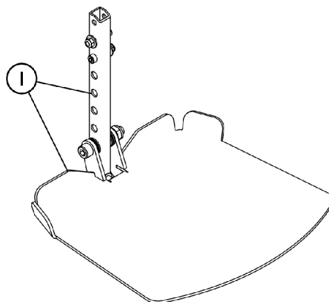
Assembled View
