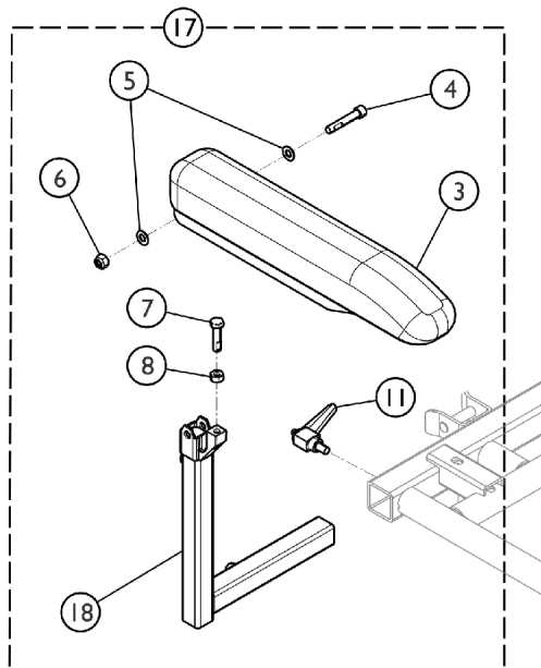
Fixed Height Arm Assembly
