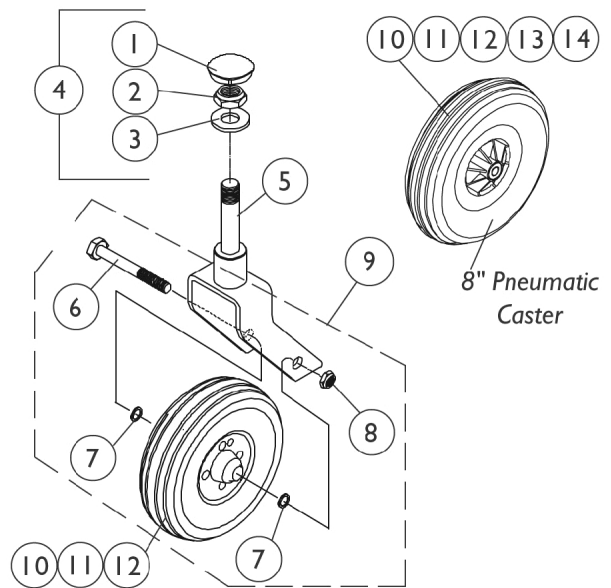
8" Caster Assembly
