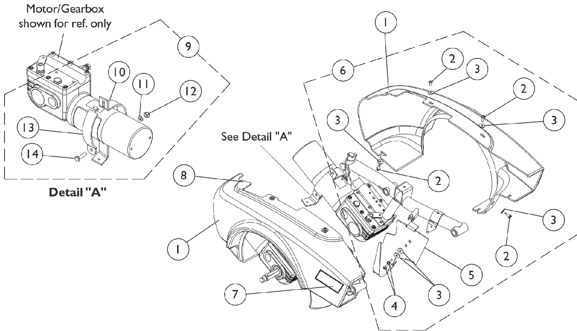
Side Shrouds
