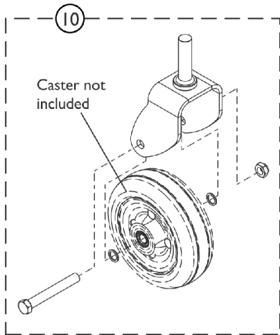
2-Sided Fork and Caster Hardware Kit (Standard)
