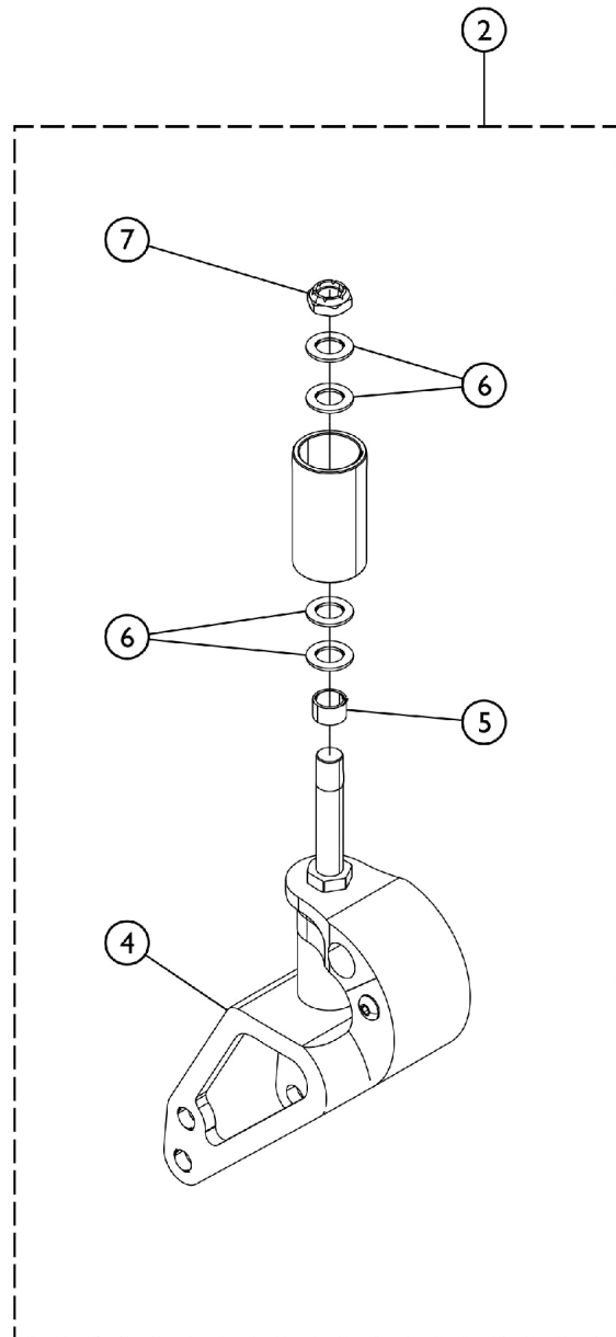
Suspension Fork for Options 1259, 8IDC, 8ID5DC All Seat to Floor Dimensions
