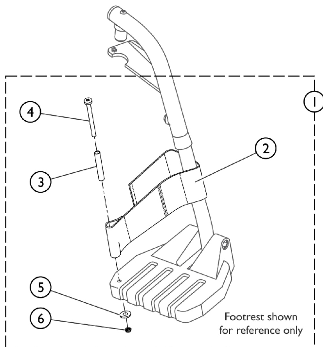
Heel Loop and Hardware for All Footplate Options with Toe Loops (1345) being used (not shown).
