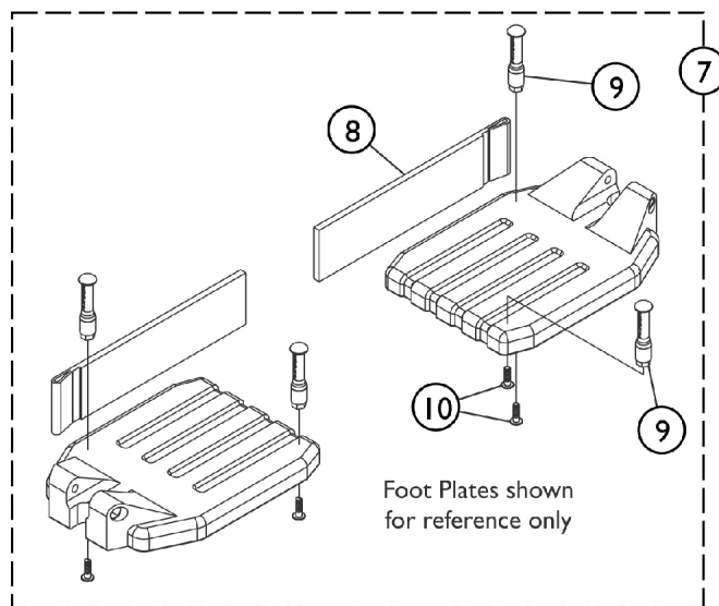
Heel Loop and Hardware for All Footplate Options without Toe Loops (1345) being used.
