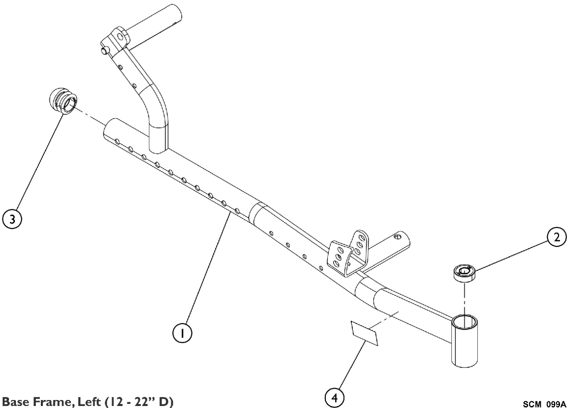
Base Frame, Left (12 - 22" D)
