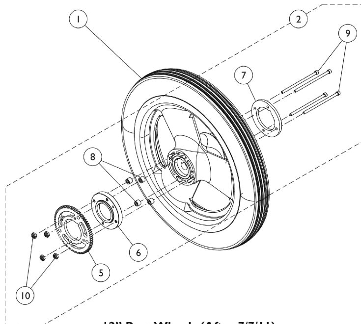
12" Rear Wheels (After 7/7/11)
