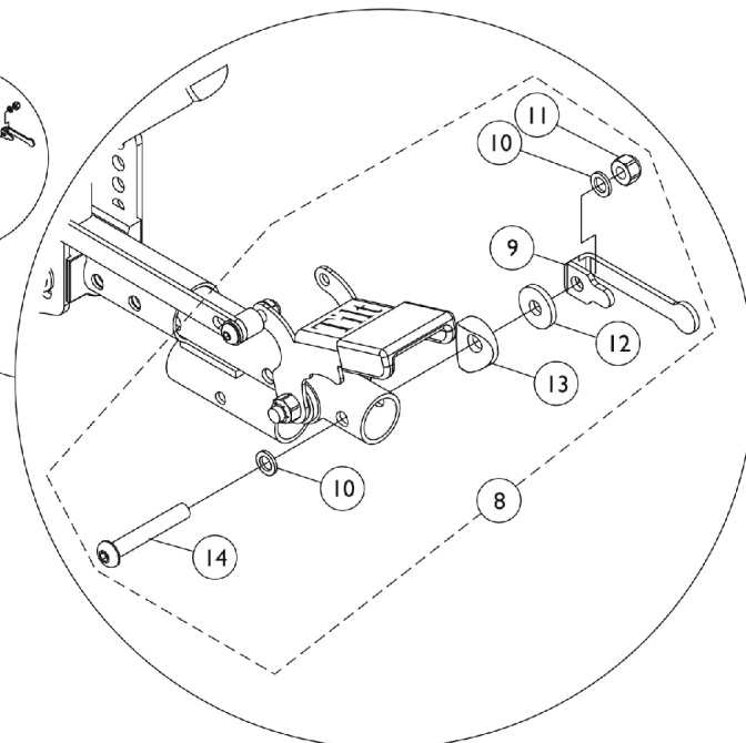
Foot Pedal Tilt Release Lockout Assembly w/ Vent Tray Option
