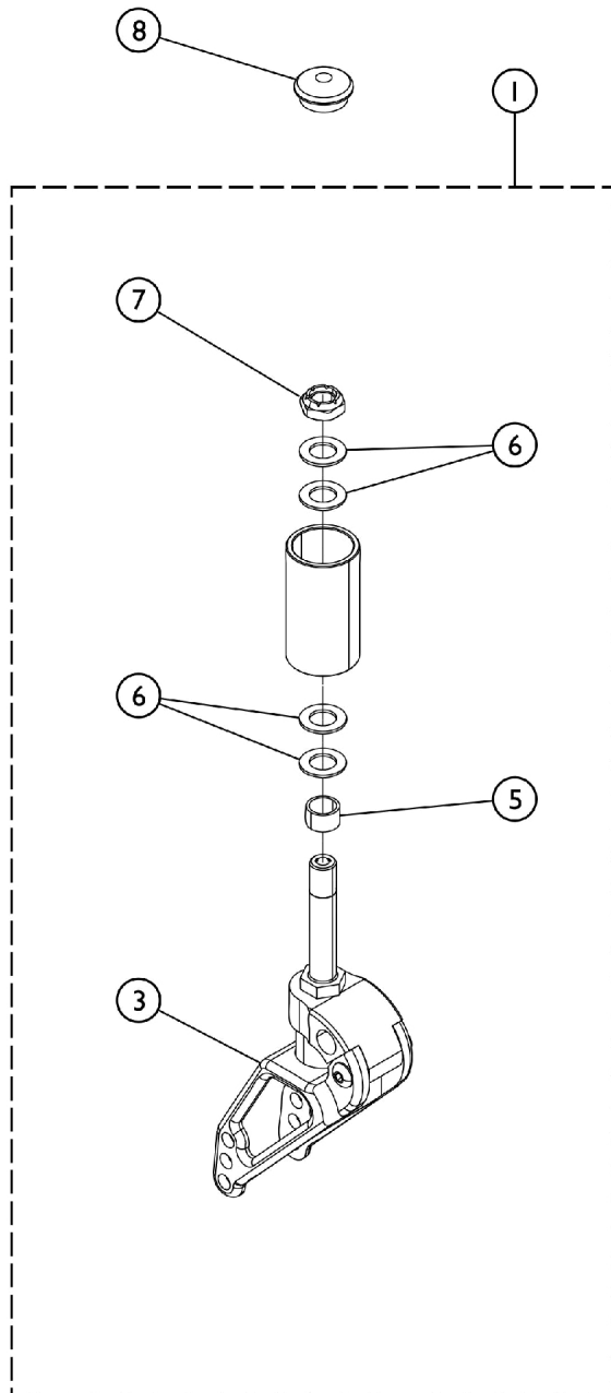
Suspension Fork for Options 4SPLT, 4ALUM2, 5IDC, 5ALUM2 5SPLT, 6IDC, 6ALUM2 All Seat to Floor Dimensions
