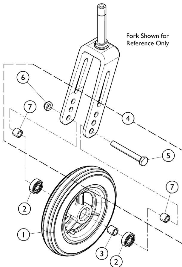
Caster and Hardware for 4SPLT, 5ALUM2, 5SOFT 5SPLT, 6ALUM2, AT902 Options
