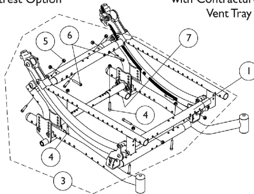
1164101 Crossbrace Tube Mounting Hardware with Heavy Duty Option
