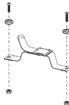
Toe Loops (For All Footplates)
