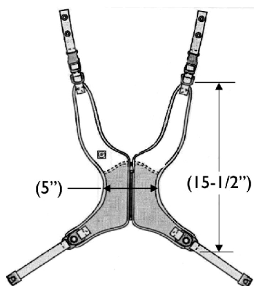
Model BPSFM 13" - 16" Wide Chairs
