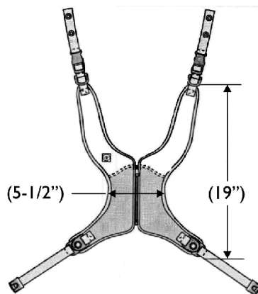
Model BPSFL 16" - 19" Wide Chairs
