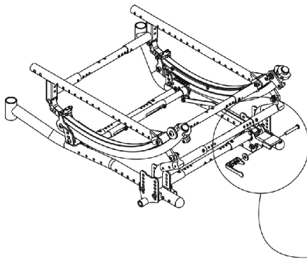
Base And Seat Frame Assembly Shown For Reference Only
