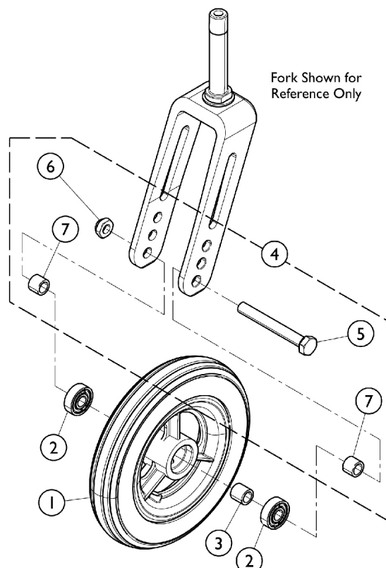
Caster and Hardware for 4SPLT, 4ALUM2, 4IDC, 4I5DC 5IDC, 5I5DC, 5ALUM2 5SPLT, 6IDC, 6I5DC Options
