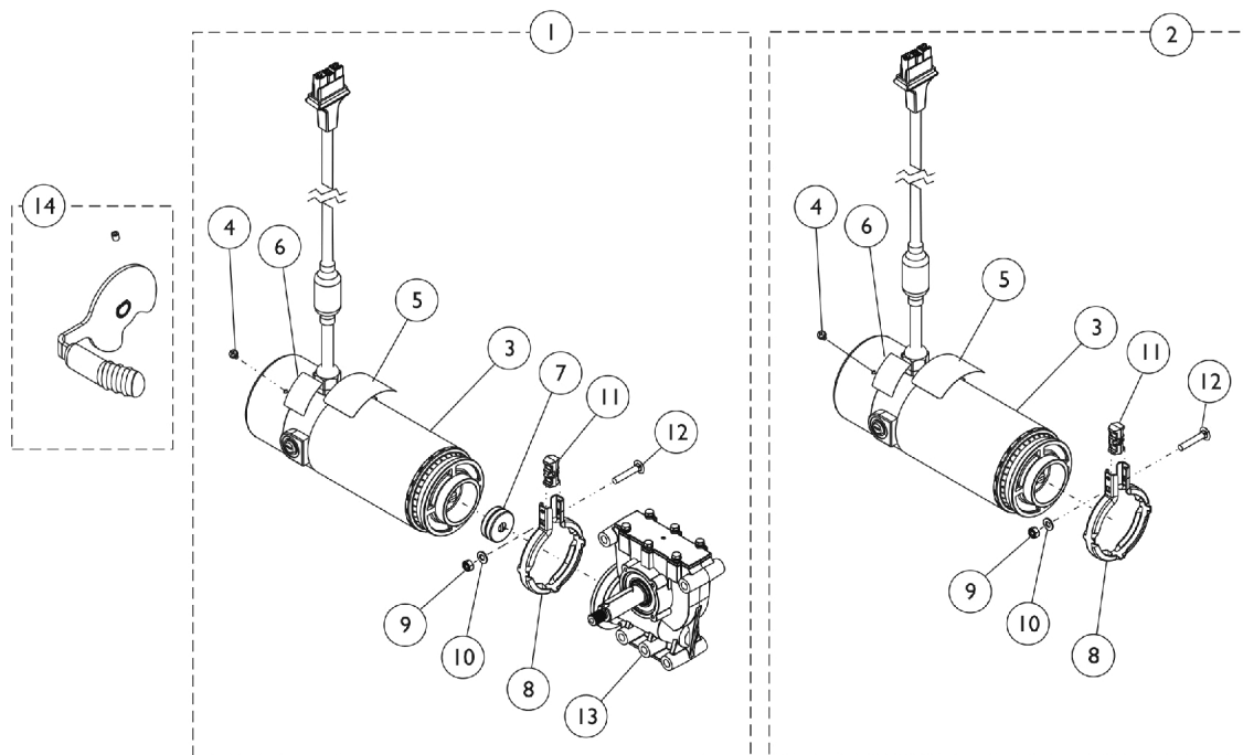
2-Pole Motor/SSD Gearbox Assembly
