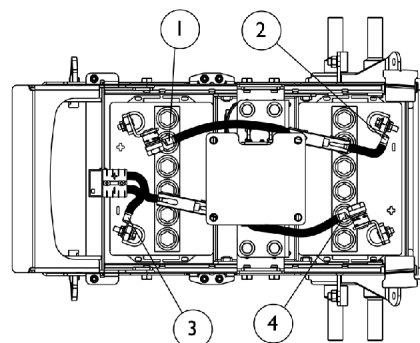
U1 Battery Installation for Elevate Configuration
