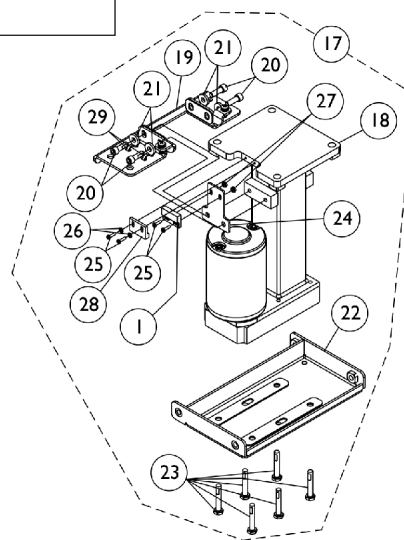
Elevate Hardware with TRBKTS Option For (TDX SC with ADJASBA Seat and CGE Option), and TDX SPREE
