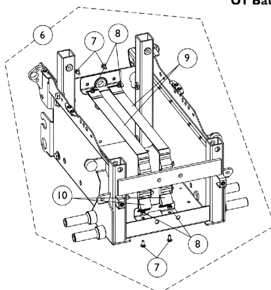
Battery Strap Assembly
