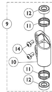
Front Head Tube Assembly
