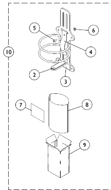
O2 Holder Home Filled Tank (HFO2-ML6)
