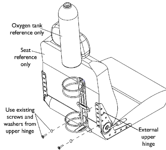
Installing on Seat with External Hinge
